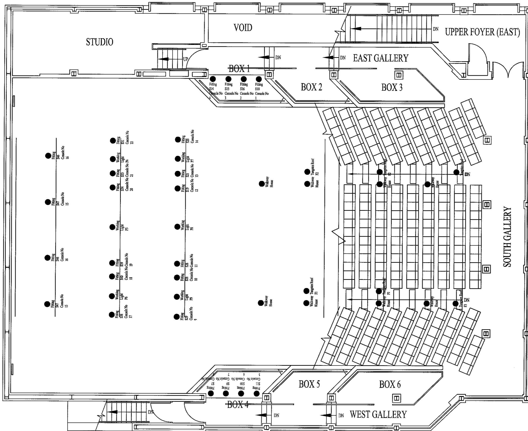
Stage lighting Standard Layout
